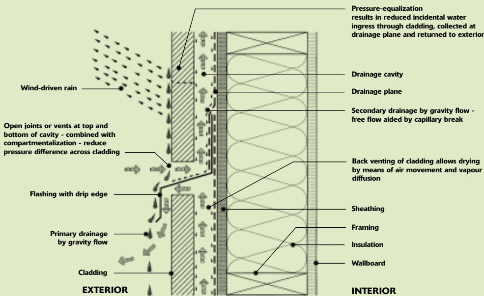
FIGURE 10: Pressure Equalizer Rainscreen Wall
