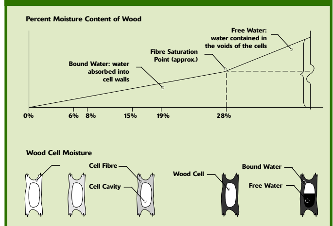
FIGURE 1: Moisture Control of Wood
